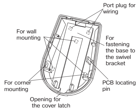
Figure 2 – Base
