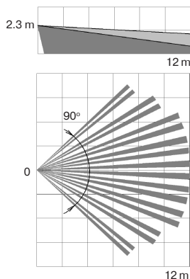
Figure 1 – Detection Zone Layout
