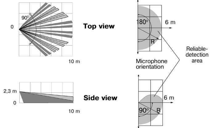
Figure 1 – PIR channel detection zone pattern
