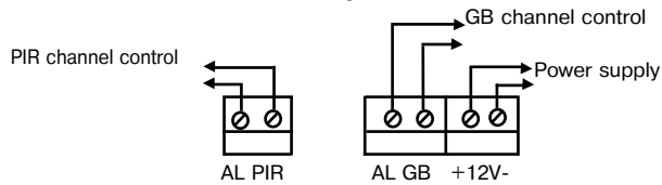
Figure 4 – The Detector connection pattern
