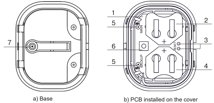
Figure 2 – The Detector Design
