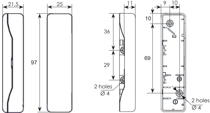
Picture 2 – Overall dimensions
