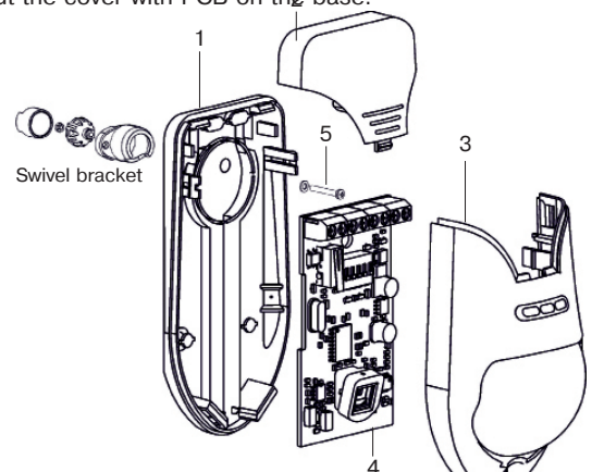
Figure 3 – Design of the Detector
