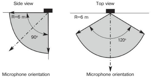
Figure 2 – GB channel detection zone pattern
