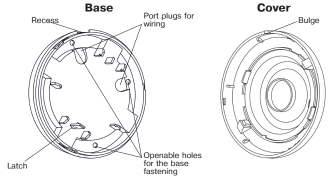
Figure 2 – Base and cover of the Detector
