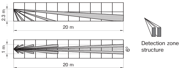
Figure 1 – Detection zone pattern
