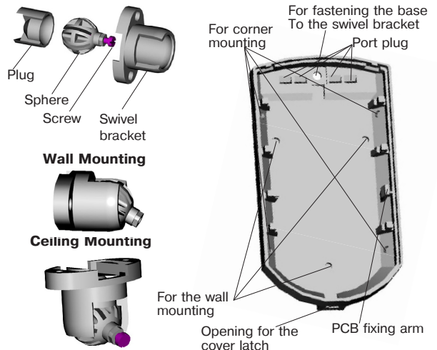
Figure 2 – The Detector Base and the Swivel Bracket
