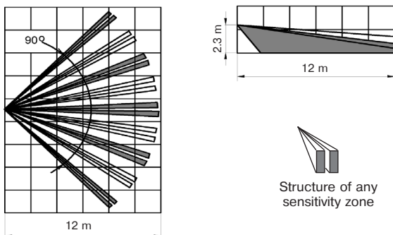
Figure 1 – Detection Zone Pattern
