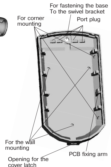
Figure 2 – The Detector Base and the Swivel Bracket
