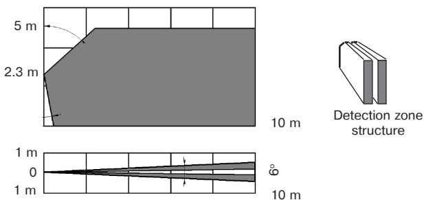
Figure 1 – Detection zone pattern
